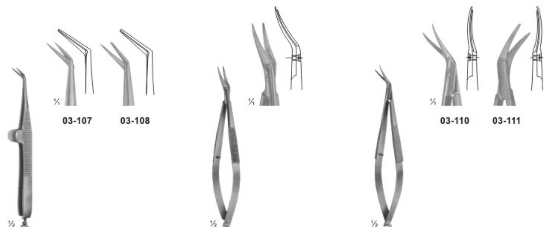
03-107 - 108 WECKER Eye scissor Size: 110 mm
